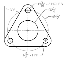
12. CARBURETOR GASKET
