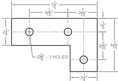
4. IDENTIFICATION PLATE
