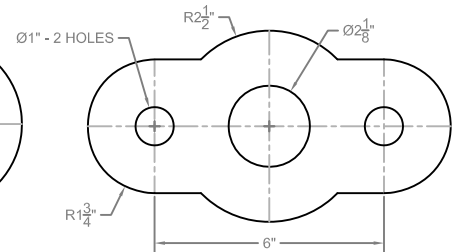
6. ROUND FLANGE
