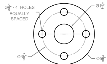
9. BASE PLATE
