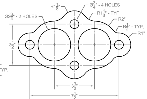
12. CARBURETOR GASKET
