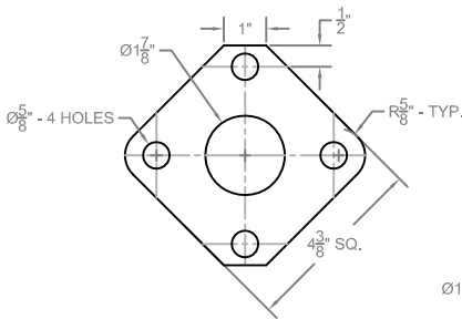
10. COVER PLATE
