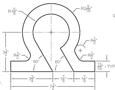
11. HOUSING
